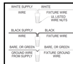
Wiring Diagram
