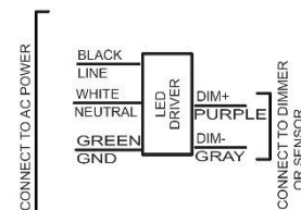
Wiring Diagram 2
