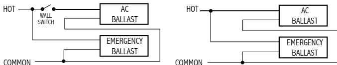
Primary circuit only. Lamp leads not shown.
