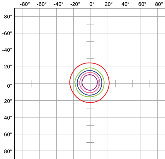
ISOCANDELA PLOT
