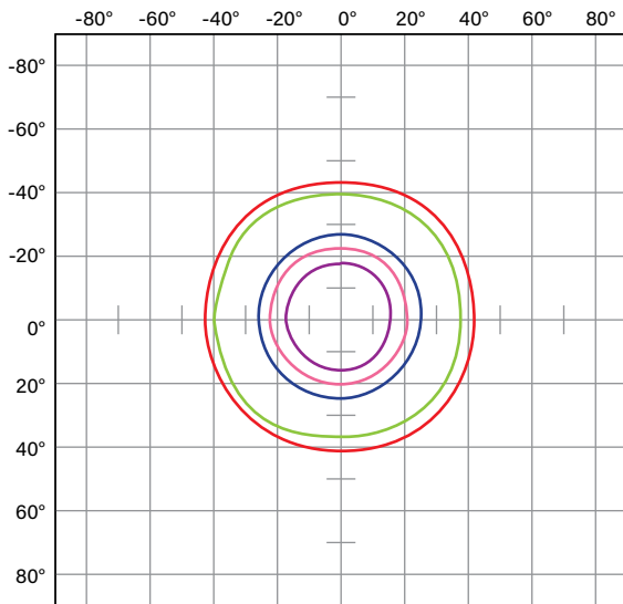
ISOCANDELA PLOT
