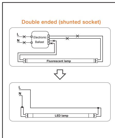
Wiring method - II
