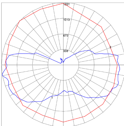
Maximum Candela = 1350.76 Located At Horizontal Angle = 135, Vertical Angle = 80 # 1 - Vertical Plane Through Horizontal Angles (135 - 315) (Through Max. Cd.) # 2 - Horizontal Cone Through Vertical Angle (80) (Through Max. Cd.)
