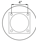
Anchor Bolt M10 x 6.5" (4 anchor bolts and template included)
