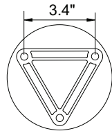
Anchor Bolt M10 x 6.5" (3 anchor bolts and template included)
