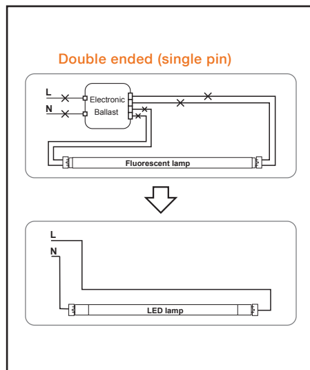
Wiring method - III
