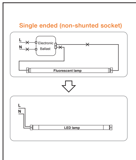
Wiring method - I
