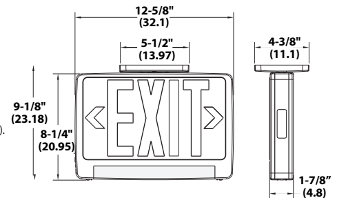
ECBR LED
